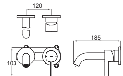
TLG11307BA Wall Mounted Single Lever Washbasin Faucet (Short Spout) Size: 120W x 185D x 103H mm
