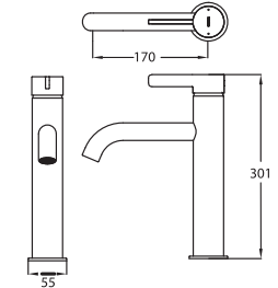
TLG11306B Single Lever Washbasin Faucet for Tall Vessel w/o Pop-Up Waste Size: 55W x 170D x 301H mm
