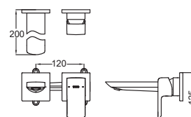
TLG02310B2 Wall Mounted Single Lever Washbasin Faucet, Exposed (Short Spout) Size: 120W x 200D x 125H mm
