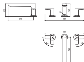
TBG13201A Bathtub Filler w/o HS(3 Hole) Size: 380W x 250D x 125H mm
