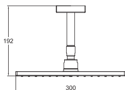
TBW08003A1 Fixed Shower Head (1 Mode) (Ceiling Type) Size: 300 mm x 300 mm
