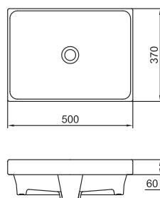
L1715#WH Console Washbasin Size: 500W x 370D x 60H mm
