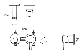
TLS02308B2 Wall Mounted Single Lever Washbasin Faucet, Exposed (Long Spout) Size: 120W x 267D x 76H mm
