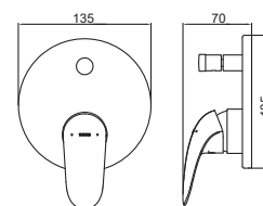
TBS03304B2 Single Lever Bath & Shower Mixer w/ Diverter and Valve Size: 135W x 70D x 135H mm
