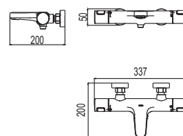
TBW09400A Thermo Expo Bath & Shower Faucet Size : 337W x 200D x 50H mm
