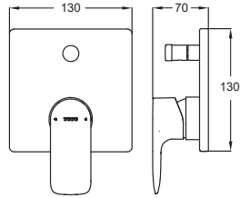
TBG04304BA Single Lever Shower Mixer w/ Diverter Size: 130W x 70D x 130H mm
