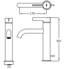
TLG11305B Single Lever Washbasin Faucet for Tall Vessel w/ Pop-Up Waste Size: 55W x 170D x 301H mm
