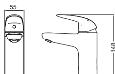
TLS03302B Single Lever Washbasin Faucet w/o Pop-Up Waste Size: 55W x 95W x 148H mm
