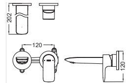
TLG04309B2 Wall Mounted Single Lever Washbasin Faucet, Exposed (Short Spout) Size: 120W x 202D x 120H mm
