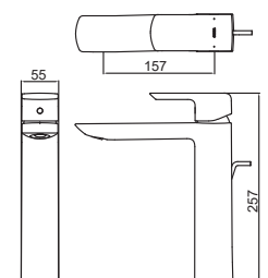
TLG02307B Single Lever Washbasin Faucet for Tall Vessel w/ Pop-Up Waste Size : 55W x 157D x 257H mm
