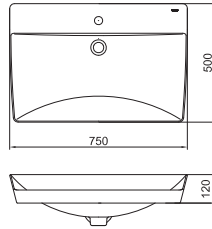
LW340CJW/F#W Console Washbasin Size: 750W x 500D x 120H mm
