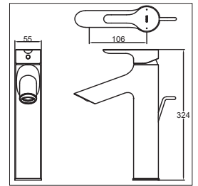
TLS01307B Single Lever Washbasin Faucet for Tall Vessel w/ Pop-up Waste Size: 55W x 106D x 324H mm
