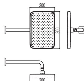
TBW10020A Over Head Shower (1 Mode) (Wall Mounted) Size : 300W x 200D mm
