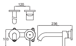
TLG11308BA Wall Mounted Single Lever Washbasin Faucet (Long Spout) Size: 120W x 236D x 103H mm
