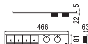
TBV11140A#BFG (Brushed French Gold)
