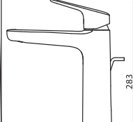
TLG03305B Single Lever Washbasin Faucet for Tall Vessel w/ Pop-Up Waste Size: 50W x 165D x 283H mm
