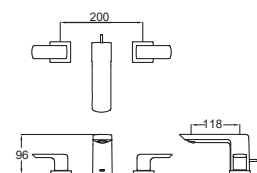
TLG02201BB 2 Handle Washbasin Faucet (3 Holes) w/ Pop-Up Waste Size: 200W x 118D x 96H mm
