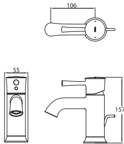
TLS02301B Single Lever Washbasin Faucet w/ Pop-Up Waste Size: 55W x 106D x 157H mm
