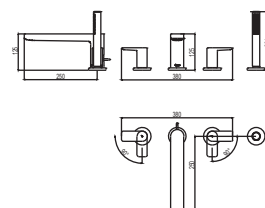
TBG13202A Bathtub Filler w/ HS (4Hole) Size: 460W x 250D x 200H mm
