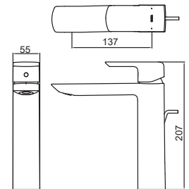
TLG02304B Single Lever Washbasin Faucet for Semi-tall Vessel w/ Pop-Up Waste Size : 55W x 137D x 207H mm
