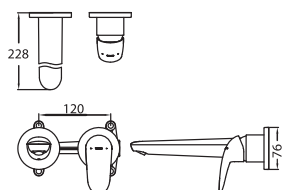
TLS03308B2 Wall Mounted Single Lever Washbasin Faucet, Exposed (Long Spout) Size: 120W x 228D x 76H mm
