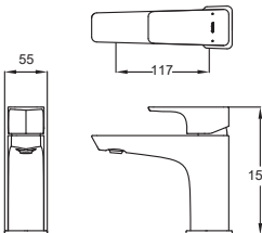
TLG07302B Single Lever Washbasin Faucet w/o Pop-Up Waste Size: 55W x 117D x 155H mm
