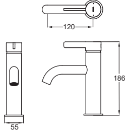
TLG11302B Single Lever Washbasin Faucet w/o Pop-Up Waste Size: 55W x 120D x 186H mm
