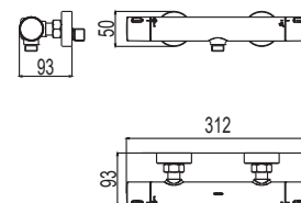
TBW09410A Thermo Expo Shower Faucet Size : 312W x 93D x 50H mm
