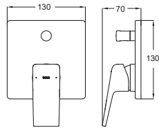
TBG10303BA Single Lever Shower Mixer Size: 130W x 70D x 130H mm
