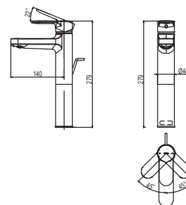
TLS06305A Single Lever Washbasin Faucet w/ Pop-up Waste Size: 44W x 140D x 279H mm
