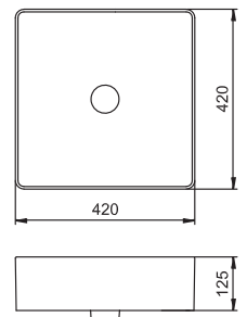
LW574JW/F#W Console Washbasin Size: 420W x 420D x 125H mm
