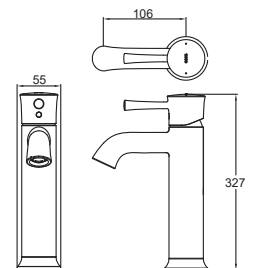
TLS02306B Single Lever Washbasin Faucet for Tall Vessel w/o Pop-Up Waste Size: 55W x 106D x 327H mm
