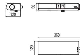
TBV10400A Touch Button Thermo Bath & Shower Size : 360W x 120D x 60H mm
