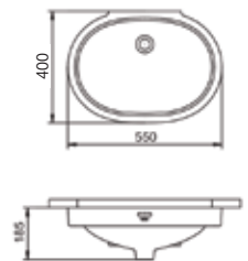
LW546M#NW1 Under Counter Washbasin Size: 550W x 400D x 185H mm
