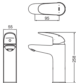
TLS03304B Single Lever Washbasin Faucet for Semi-tall Vessel w/o Pop-Up Waste Size: 55W x 95D x 258H mm
