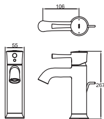
TLS02303B Single Lever Washbasin Faucet for Semi-tall Vessel w/ Pop-Up Waste Size: 55W x 106D x 267H mm
