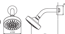
TBW01013B Fixed Shower Head (Wall Type) (Multi Mode) Size : Dia 102 mm
