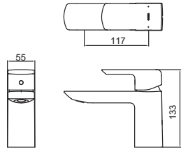
TLG02303B Single Lever Washbasin Faucet w/o Pop-Up Waste Size : 55W x 117D x 133H mm
