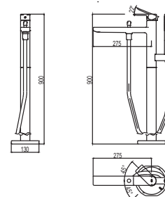
TBG13306A Floor Mount Bathtub Filler w/ HS Size: 130W x 275D x 900H mm
