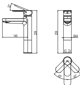
Single Lever Washbasin Faucet w/o Pop-up Waste Size: 44W x 140D x 239H mm
