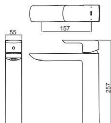
TLG02308B Single Lever Washbasin Faucet for Tall Vessel w/o Pop-Up Waste Size : 55W x 157D x 257H mm
