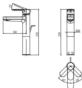
Single Lever Washbasin Faucet w/o Pop-up Waste Size: 44W x 140D x 279H mm
