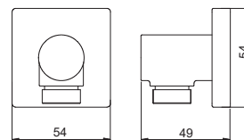
TBW02013B Wall Outlet Size : 54W x 49D x 54H mm
