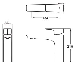
TLG07304B Single Lever Washbasin Faucet for Semi-tall Vessel w/o Pop-Up Waste Size: 55W x 134D x 215H mm
