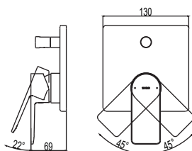
TBG13304A Concealed Bath & Shower Mixer Size: 130W x 69D x 150H mm
