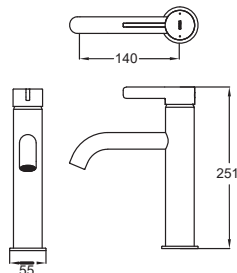
TLG11304B Single Lever Washbasin Faucet for Semi-tall Vessel w/o Pop-Up Waste Size: 55W x 140D x 251H mm
