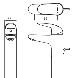
TLS03305B Single Lever Washbasin Faucet for Tall Vessel w/ Pop-Up Waste Size: 55W x 95D x 318H mm
