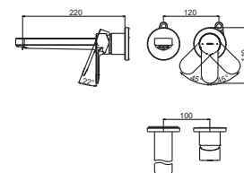
Single Lever Washbasin Faucet Wall Mounted (Long Spout) Size: 120W x 220D x 110H mm
