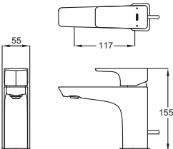
TLG07301B Single Lever Washbasin Faucet w/ Pop-Up Waste Size: 55W x 117D x 155H mm
