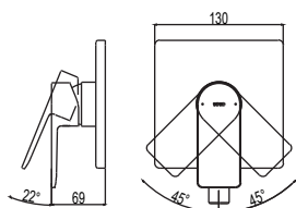
TBG13303A Concealed Shower Mixer Size : 130W x 69D x 150H mm
