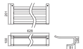
YTS903BC Towel Shelf Size: 628W x 201D x 100H mm
