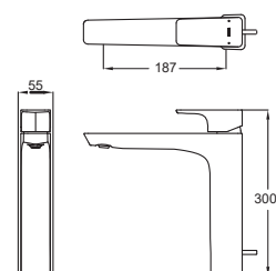
TLG07305B Single Lever Washbasin Faucet for Tall Vessel w/ Pop-Up Waste Size: 55W x 187D x 300H mm
