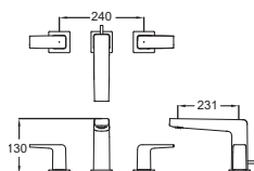
TBG10201B Bath Filler w/o Shower (3 Holes) Size: 240W x 231D x 130H mm
