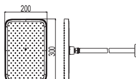
TBW10030A Over Head Shower (1 Mode) (Ceiling Mounted) Size : 300W x 200D mm
