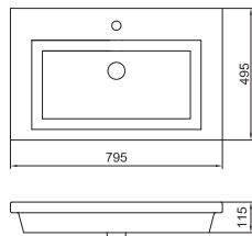
LW648CJW/F#W Console Washbasin 1 Tap Hole Size: 795W x 495D x 115H mm
