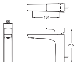
TLG07303B Single Lever Washbasin Faucet for Semi-tall Vessel w/ Pop-Up Waste Size: 55W x 134D x 215H mm
