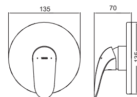
TBS03303B2 Single Lever Shower Mixer w/ Valve Size: 135W x 70D x 135H mm
