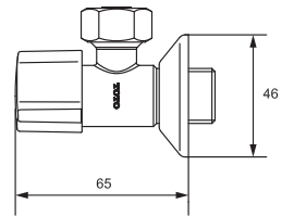
TX277SV1 Stop Valve w/o Flexible Hose Size: 65D x 46H mm
