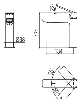
TLG13302A Single Lever Washbasin Faucet w/o Pop-U(S) Size: 38W x 134D x 171H mm
