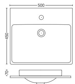
L710CSRE#XW Console Washbasin Size: 500W x 450D x 70H mm
