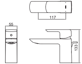
TLG02301B Single Lever Washbasin Faucet w/ Pop-Up Waste Size : 55W x 117D x 133H mm
