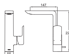
TLG02309BB Single Lever Washbasin Faucet (Side Handle) w/ Pop-Up Waste Size: 55W x 147D x 220H mm
