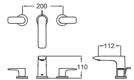
TLG04201BB 2 Handle Washbasin Faucet (3 Holes) w/ Pop-Up Waste Size: 200W x 112D x 110H mm
