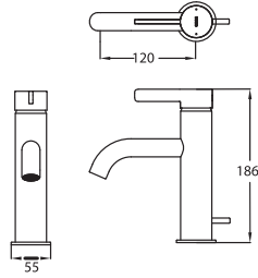
TLG11301B Single Lever Washbasin Faucet w/ Pop-Up Waste Size: 55W x 120D x 186H mm
