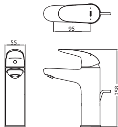
TLS03303B Single Lever Washbasin Faucet for Semi-tall Vessel w/ Pop-Up Waste Size: 55W x 95D x 258H mm
