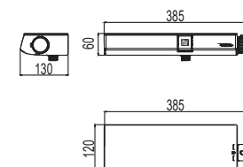
TBV10410A Touch Button Thermo Bath & Shower Size : 385W x 120D x 60H mm
