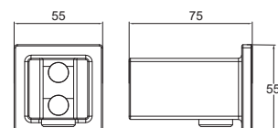
TBW08010A Wall Outlet With Shower Hanger Size: 55 x 55 mm
