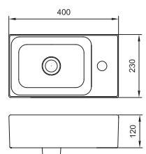
L1634#WH Console Washbasin Size: 400W x 230D x 120H mm
