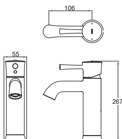
TLS02304B Single Lever Washbasin Faucet for Semi-tall Vessel w/o Pop-Up Waste Size: 55W x 106D x 267H mm
