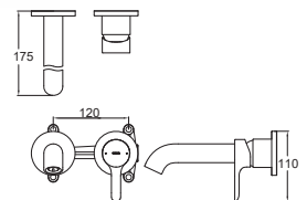
TLS01309B2 Wall Mounted Single Lever Washbasin Faucet, Exposed (Short Spout) Size: 120W x 175D x 110H mm
