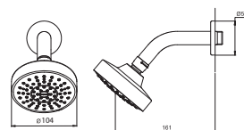
TBW03001B Fixed Shower Head (Wall Type) (Multi Mode) Size : Dia 104 mm
