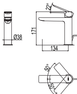
TLG13301A Single Lever Washbasin Faucet w/ Pop-U (S) Size: 38W x 134D x 171H mm
