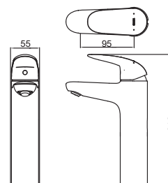
TLS03306B Single Lever Washbasin Faucet for Tall Vessel w/o Pop-Up Waste Size: 55W x 95D x 318H mm
