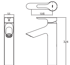
TLS01308B Single Lever Washbasin Faucet for Tall Vessel w/o Pop-Up Waste Size: 55W x 106D x 324H mm
