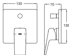
TBG10304BA Single Lever Shower Mixer w/ Diverter Size: 130W x 70D x 130H mm
