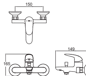
TBS03302B Single Lever Bath & Shower Mixer Size: 150W x 149D x 165H mm
