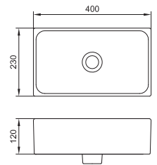
L1734#WH Console Washbasin Size: 400W x 230D x 120H mm
