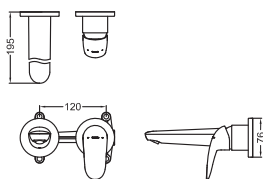
TLS03307B2 Wall Mounted Single Lever Washbasin Faucet, Exposed (Short Spout) Size: 120W x 195D x 76H mm
