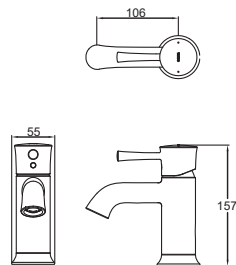
TLS02302B Single Lever Washbasin Faucet w/o Pop-Up Waste Size: 55W x 106D x 157H mm
