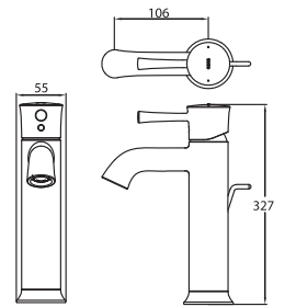
TLS02305B Single Lever Washbasin Faucet for Tall Vessel w/ Pop-Up Waste Size : 55W x 106D x 327H mm
