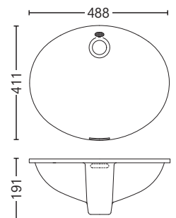
LW569M#NW1 Under Counter Washbasin Size: 488W x 411D x 191H mm
