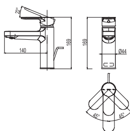
TLS06301A Single Lever Washbasin Faucet w/ Pop-up Waste Size: 44W x 140D x 169H mm
