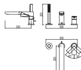
TBG13305A Bathtub Filler w/ HS (3 Hole) Size: 300W x 250D x 200H mm
