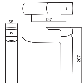
TLG02306B Single Lever Washbasin Faucet for Semi-tall Vessel w/o Pop-Up Waste Size : 55W x 137D x 207H mm
