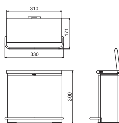
YKB102 Dust Box Size: 330 W x 171 D x 300 H x mm
