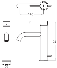
TLG11303B Single Lever Washbasin Faucet for Semi-tall Vessel w/ Pop-Up Waste Size: 55W x 140D x 251H mm
