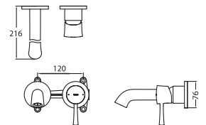
TLS02307B2 Wall Mounted Single Lever Washbasin Faucet, Exposed (Short Spout) Size: 120W x 216D x 76H mm
