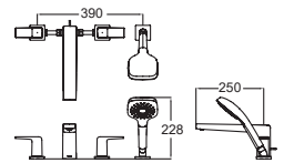
TBG10202A Bath & Shower Set (4 Holes) Size: 390W x 250D x 228H mm
