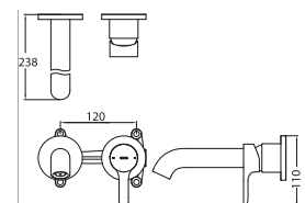
TLS01310B2 Wall Mounted Single Lever Washbasin Faucet, Exposed (Long Spout) Size: 120W x 238D x 110H mm
