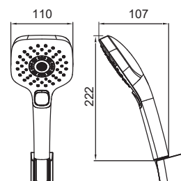
TBW02006A#PFG (Polished French Gold)
