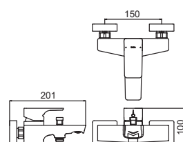
TBG07302BA Single Lever Bath & Shower Mixer Size: 150W x 201D x 100H mm
