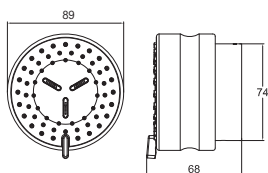
TBW07017A Body Shower (2 Mode) Size : 89W x 68D x 89H mm
