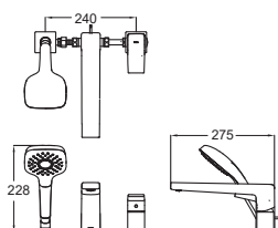
TBG10305BB Bath & Shower Set (3 Holes) Size: 240W x 275D x 228H mm
