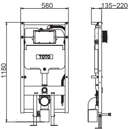
WH172AAT Concealed Tank W/Auto Flush w/ Frame water use (4.5L/3L) Size: 580W x 1180H mm
