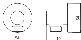
TBW01014B Wall Outlet Size : 54W x 49D x 54H mm
