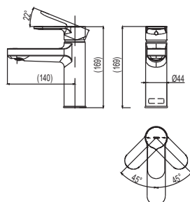
TLS06302A Single Lever Washbasin Faucet w/o Pop-up Waste Size: 44W x 140D x 169H mm
