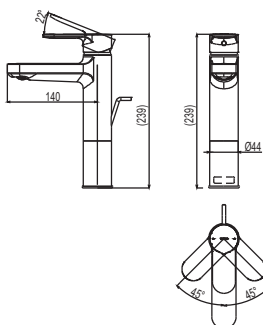
Single Lever Washbasin Faucet w/ Pop-up Waste Size: 44W x 140D x 239H mm
