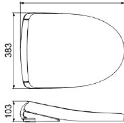
TCF47360GIN#NW1 WASHLET S7 Bowl Shape : Elongated Size : 383W x 530D x 103H mm
