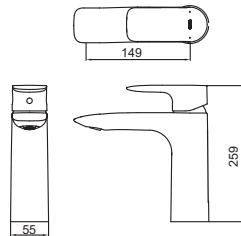
TLG04308B Single Lever Washbasin Faucet for Tall Vessel, Exposed w/o Pop-Up Waste Size: 55W x 149D x 259H mm
