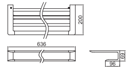
YTS902BC Towel Shelf Size: 636W x 200D x 69H mm
