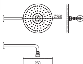
TBW10000A Over Head Shower (1 Mode) (Wall Mounted) Size : Dia 250 mm
