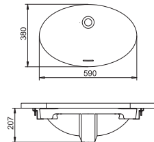
LW1506JU#W Under Counter Washbasin Size: 590W x 380D x 207H mm
