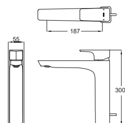
TLG07306B Single Lever Washbasin Faucet for Tall Vessel w/o Pop-Up Waste Size: 55W x 187D x 300H mm
