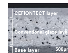
CEFIONTECT toilet micrograph *1µm=0.001mm
