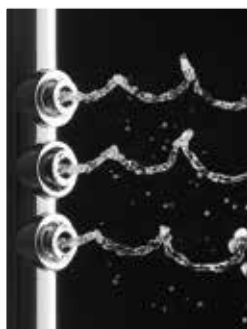
Gyrostream
